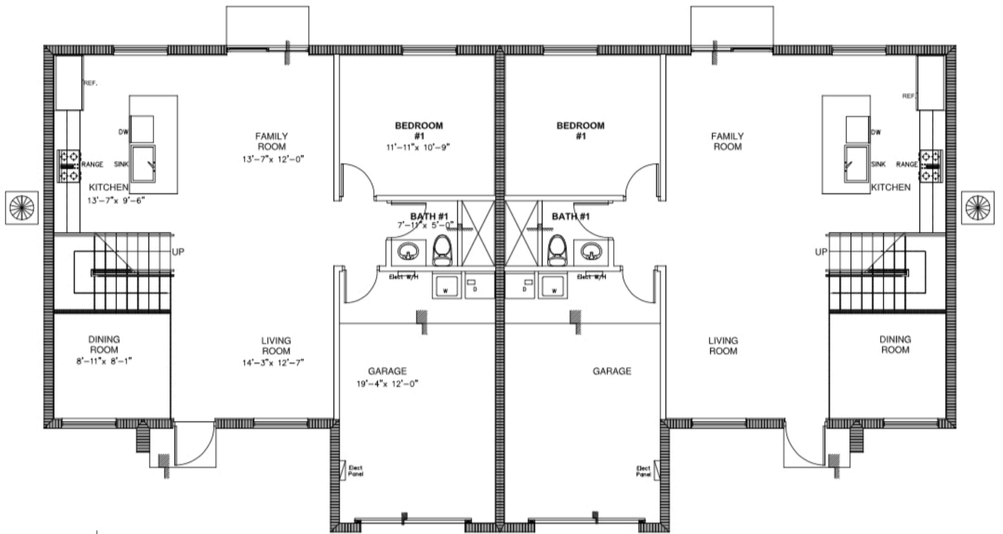
Floor Plan | Ground floor
